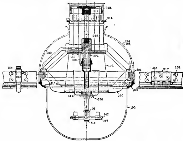
Fig. 3242. STANDARD LAMP-BODY.
